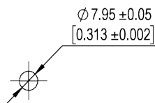
PLUG-IN MATING HOLE
